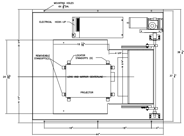
Without Plenum Cover
